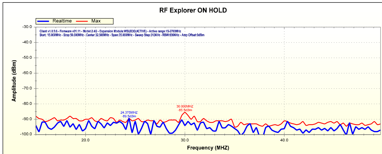
Figure 1 Lathe OFF - base line noise
