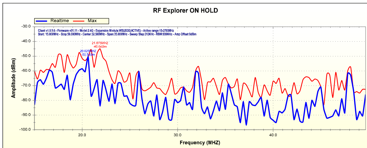
Figure 4 Lathe ON, 680 RPM
