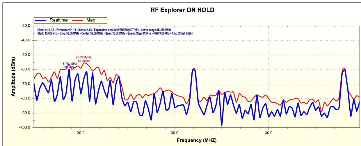
Figure 2 Lathe ON, Zero RPM
